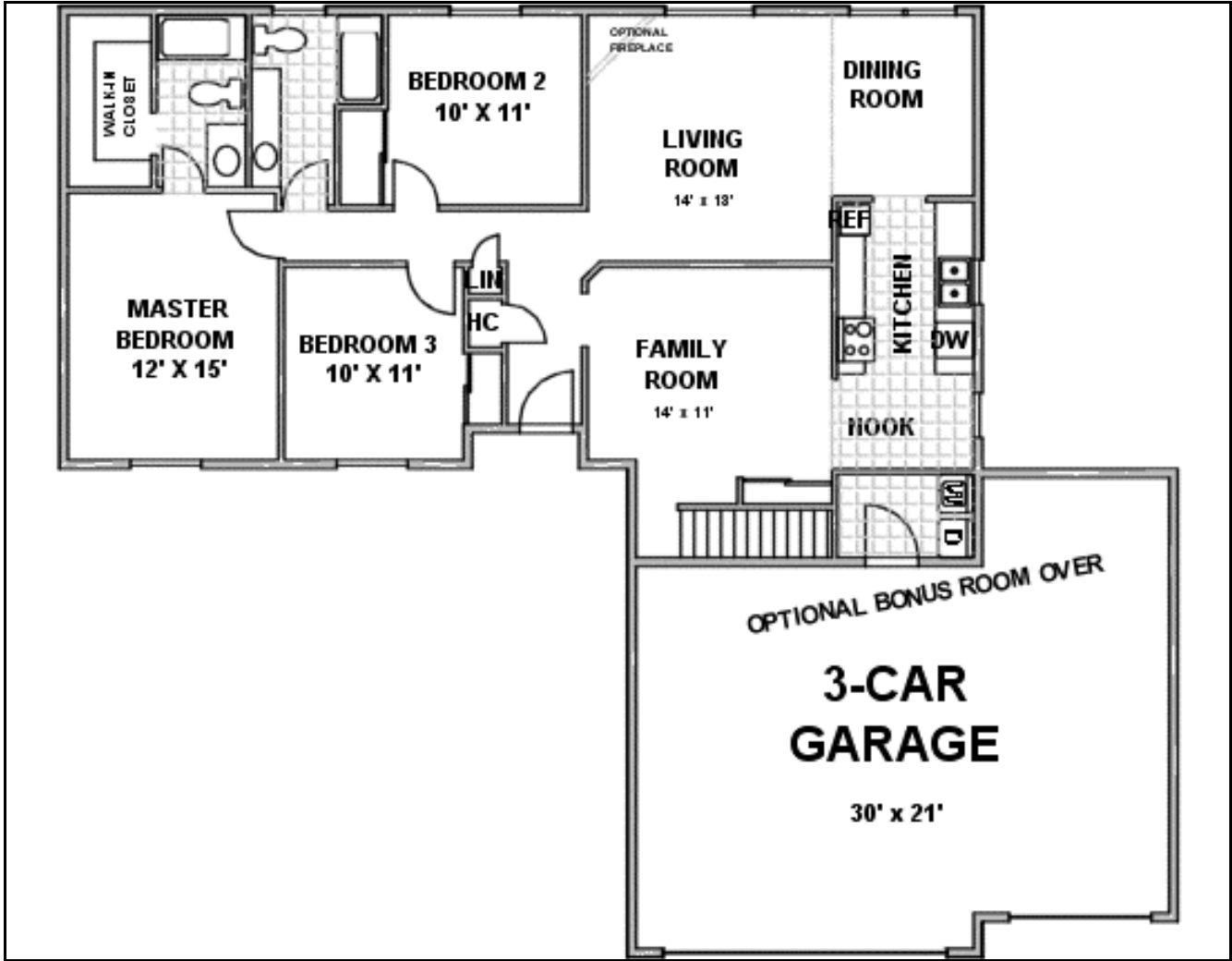
1432-03 Sq Ft Single Floor Plan
