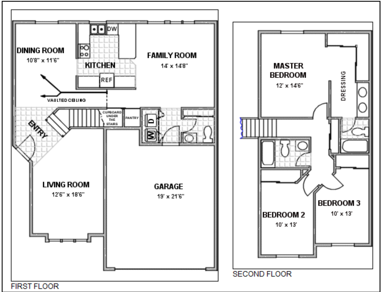
1779 Sq Ft Two Story Floor Plan
